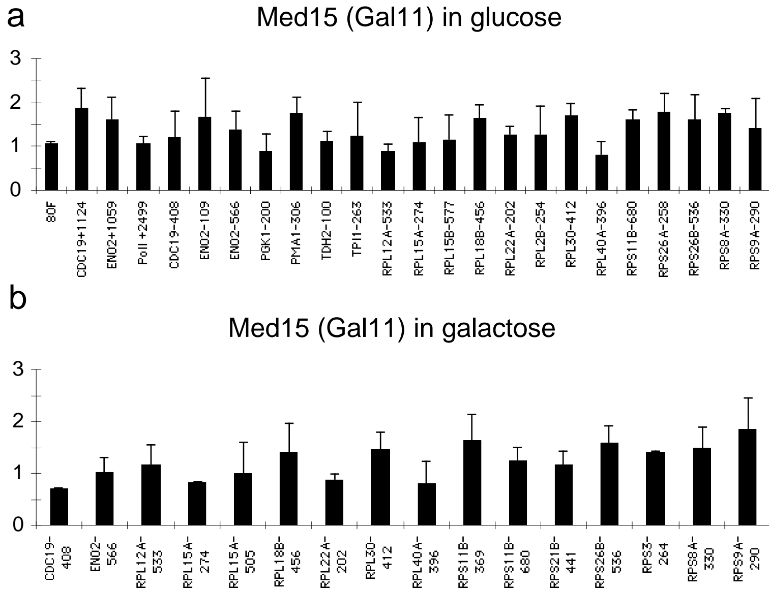
Figure S1 Mediator does not associate with transcriptionally actively ribosomal protein genes and glycolytic genes. (a-b) Occupancy of Med15 at different ribosomal protein genes and glycolytic genes when cells were grown in glucose (a) or galactose (b) .
