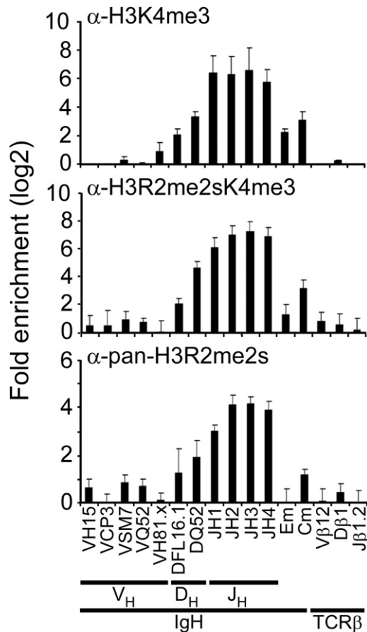
Figure 1. H3R2me2s Colocalizes with H3K4me3 at the IgH Locus in Rag2 -/- pro-B Cells
