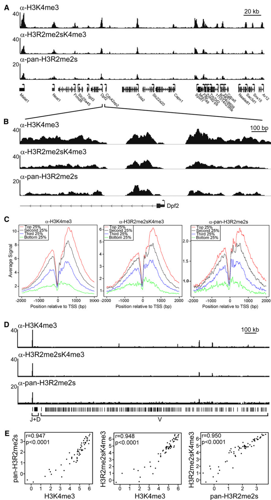
Figure 2. H3R2me2s, H3R2me2sK4me3, and H3K4me3 Are Colocalized throughout the Mouse Genome
